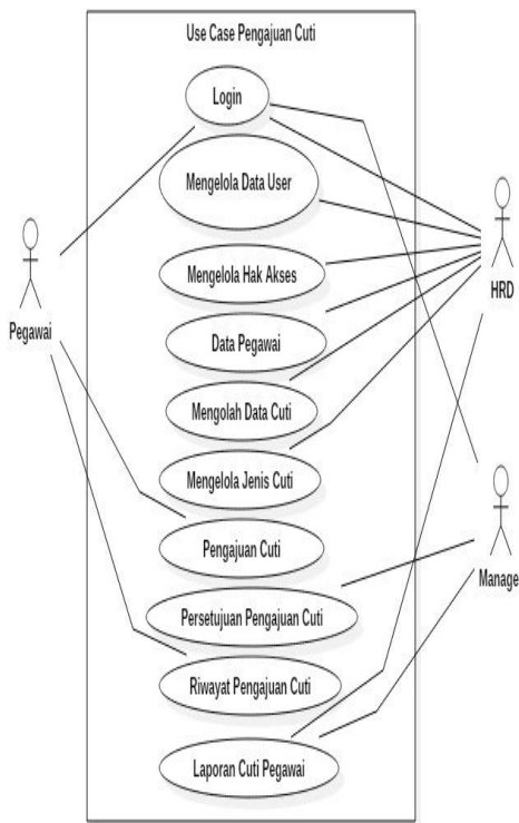
Gambar 3.3 Use Case Diagram Pengajuan Cuti
