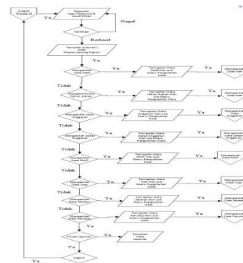
Gambar 3 Flowchart Program
