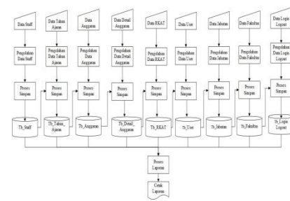
Gambar 4 Flowchart Sistem
