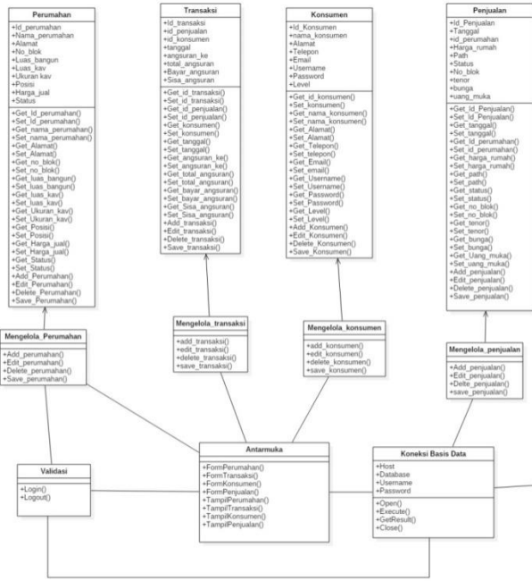
Gambar 3.4 Class Diagram
