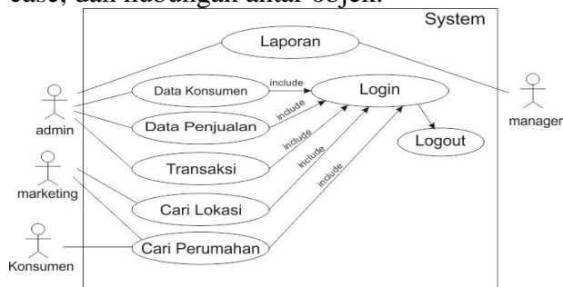
Gambar 3.3 Use case Diagram
