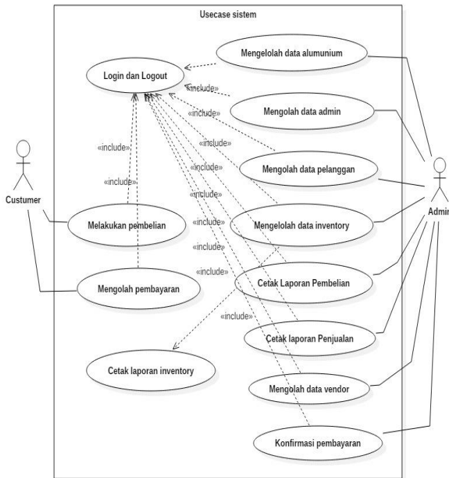
Gambar 3.3 Diagram Use case
