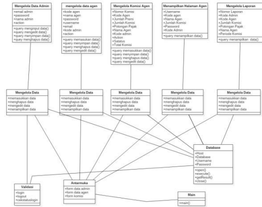
Gambar 3.4 Class Diagram
