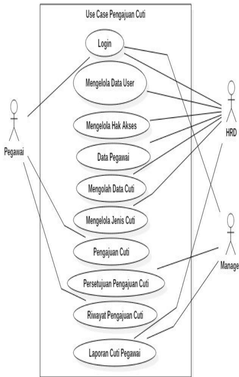
Gambar 3.3 Use Case Diagram Pengajuan Cuti
